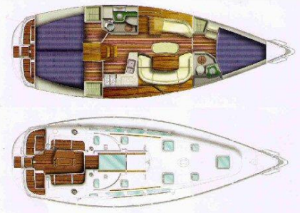
Jeanneau Sun Odyssey 40.3 "ARIES"
